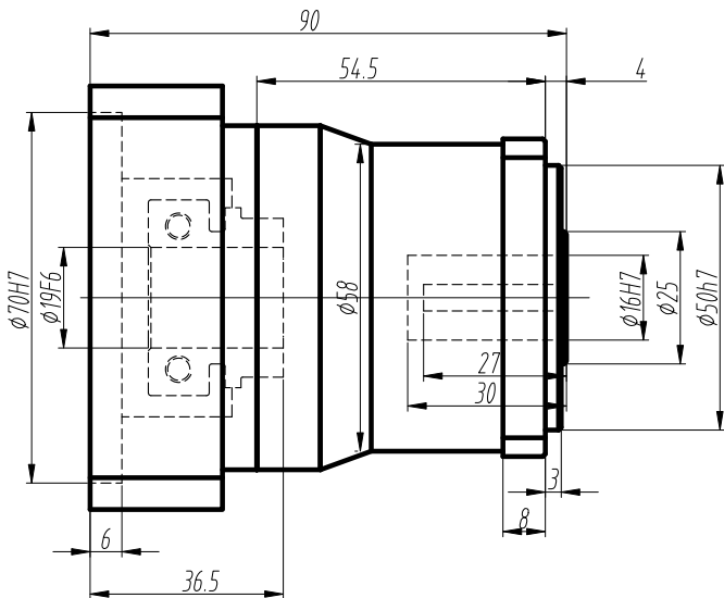
标准轴 Standard output shaft
